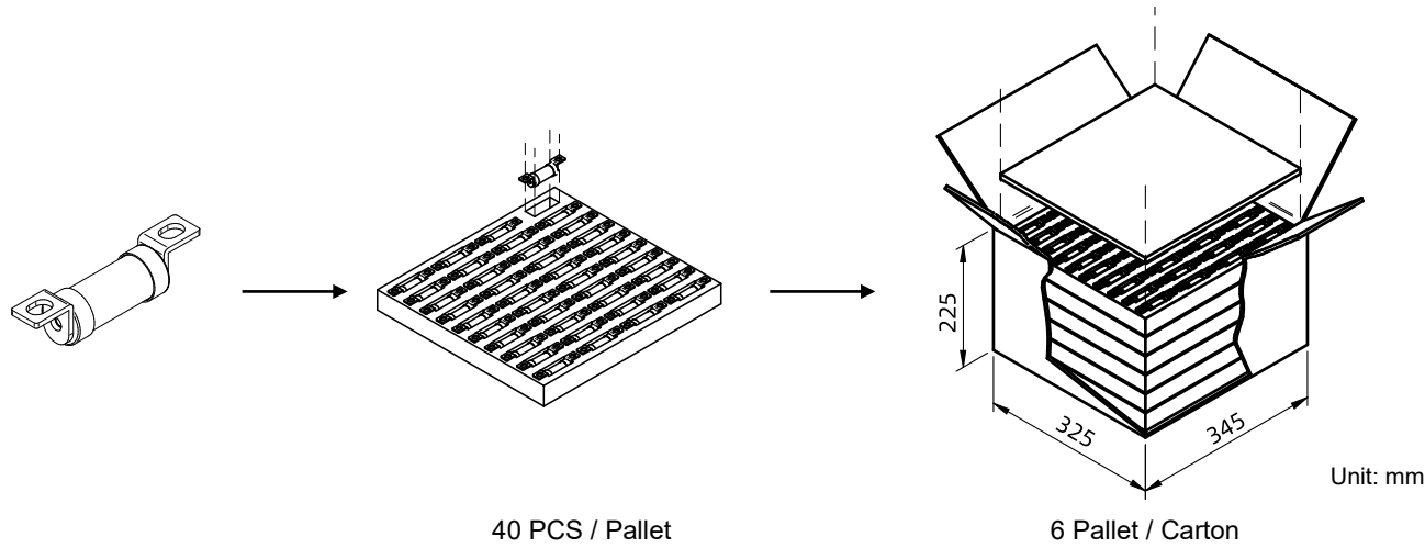
Packaging Drawing:
